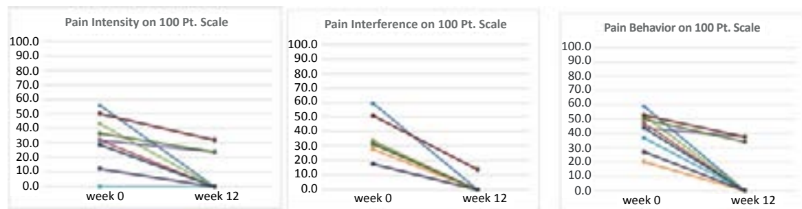
Figure 3: PROMIS pain scale results, showing all 3 metrics transformed to 100-point scale.
